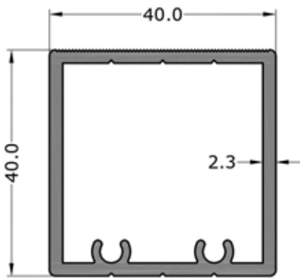
3275 0.979 KG/M (2.3 MM)
