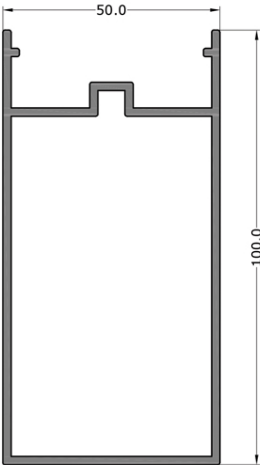
3314 1.577 KG/M (1.9 MM)
