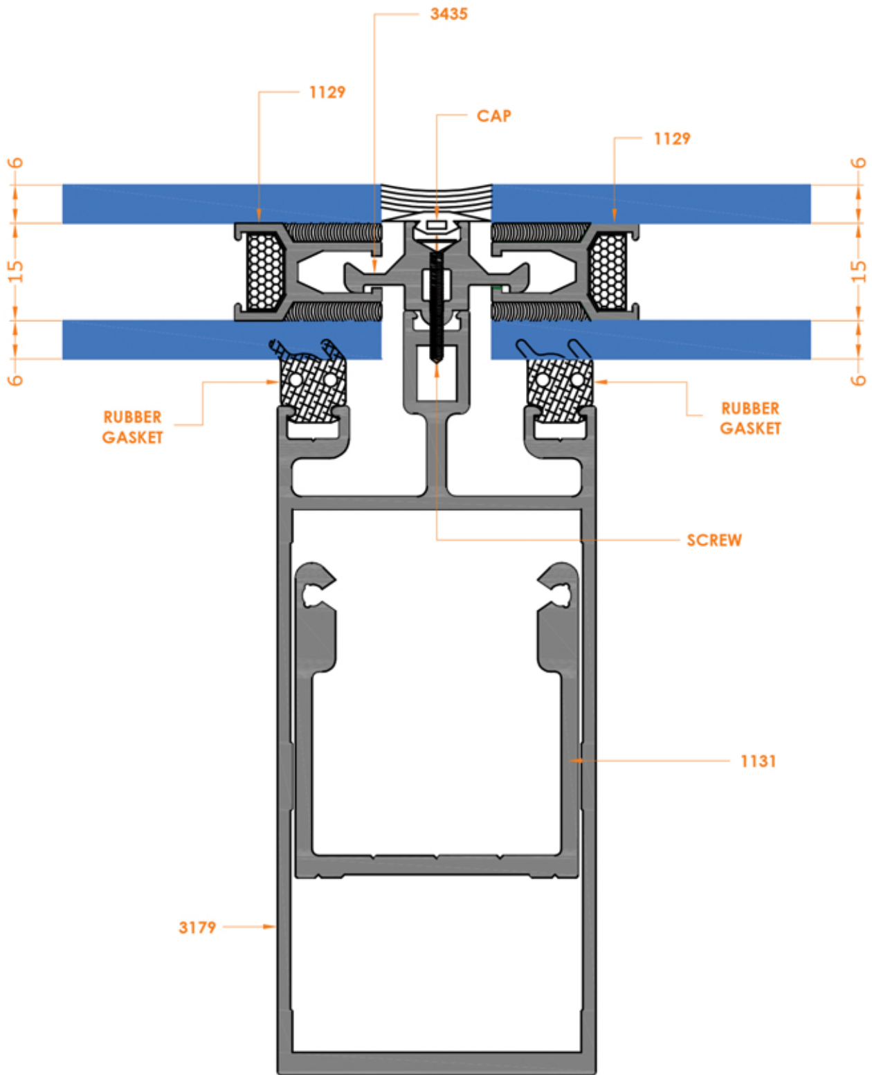
DETAILS 'B'
