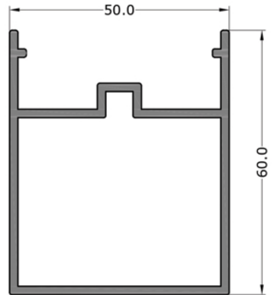
3276 1.167 KG/M (1.9 MM)
