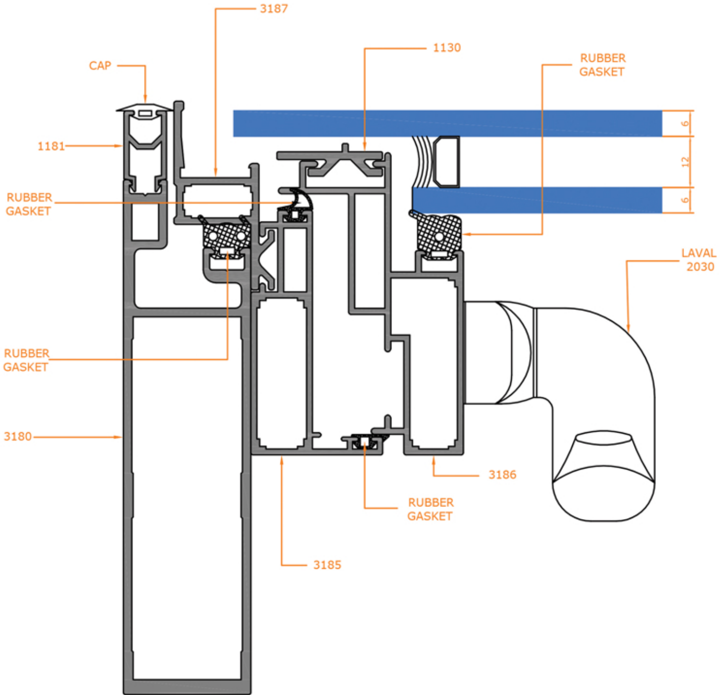
DETAILS 'D'
