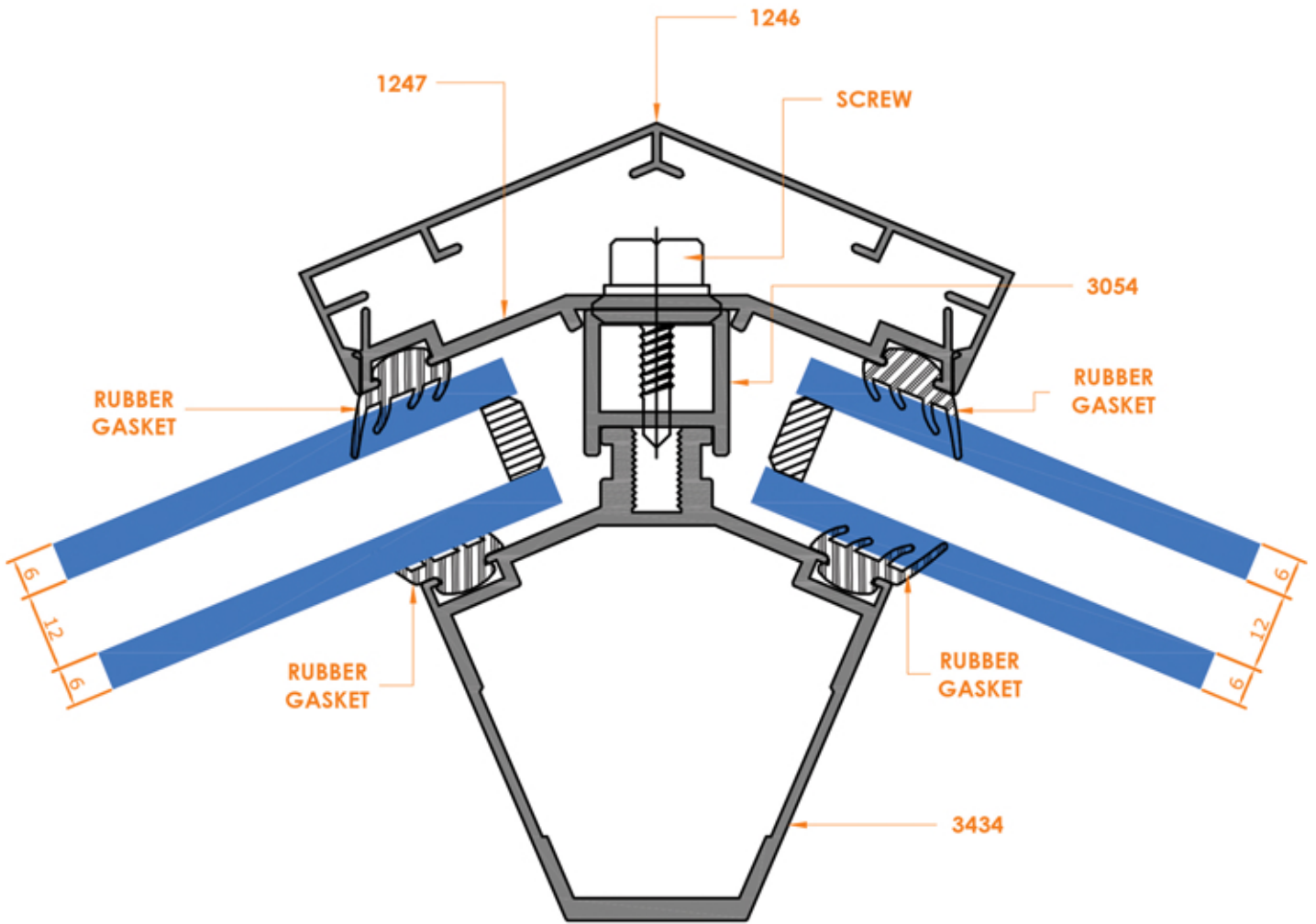
DETAILS 'A'
