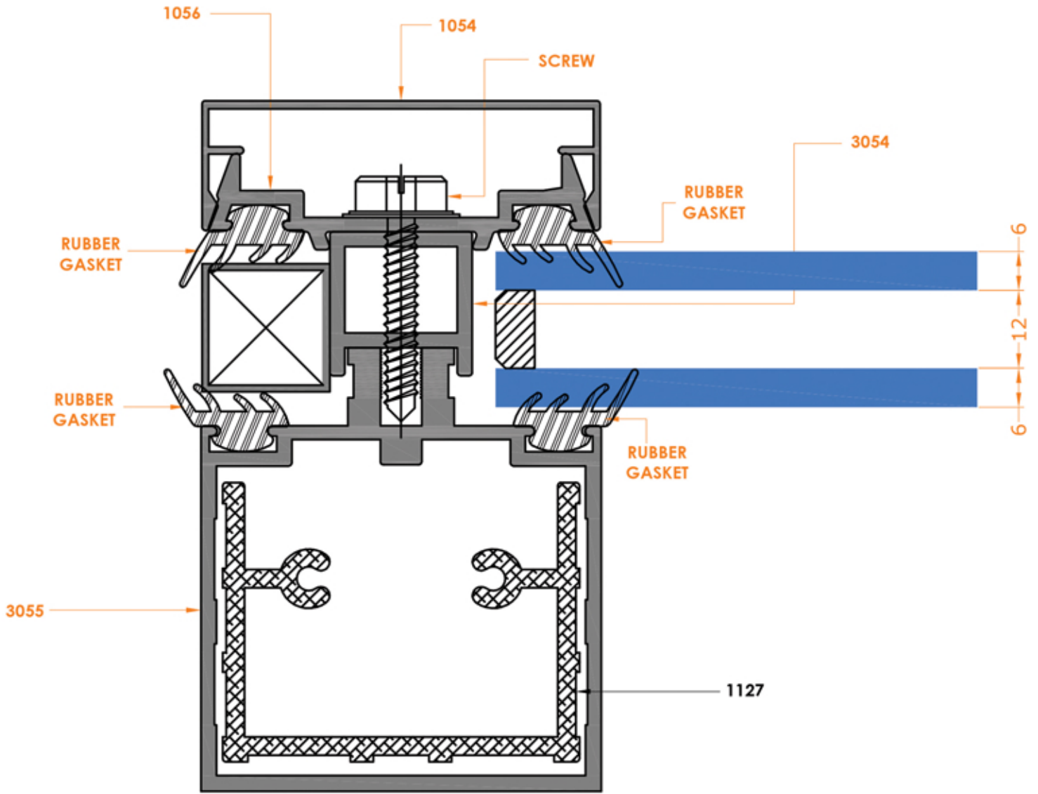
DETAILS 'B'
